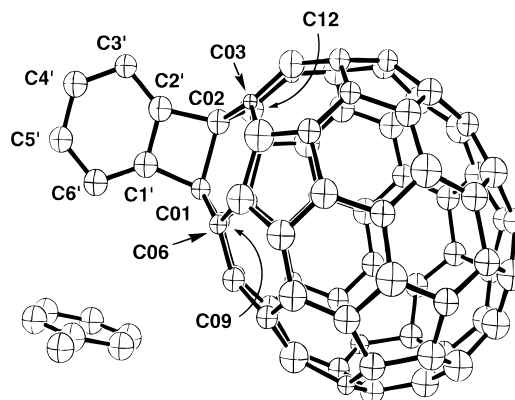
Figure 4. SHELXL-93 perspective drawing of C_{70}C_6H_4\cdot toluene ( 1a ). The shapes of the ellipsoids correspond to 50% probability contours of atomic displacement. Hydrogen atoms have been omitted for clarity.
